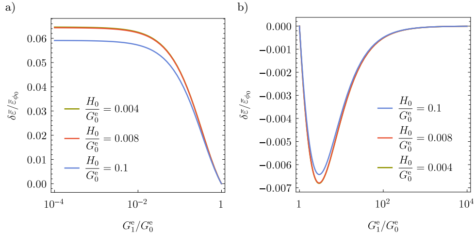
FIG. 6. Normalized strain gap \delta\bar{\varepsilon}/\bar{\varepsilon}_{\phi_0} corresponding to the mid-point rule (4.1) for \theta = 0.5 : a) G_1^{\text{e}}/G_0^{\text{e}} \leq 1 and b) G_1^{\text{e}}/G_0^{\text{e}} \geq 1 .
