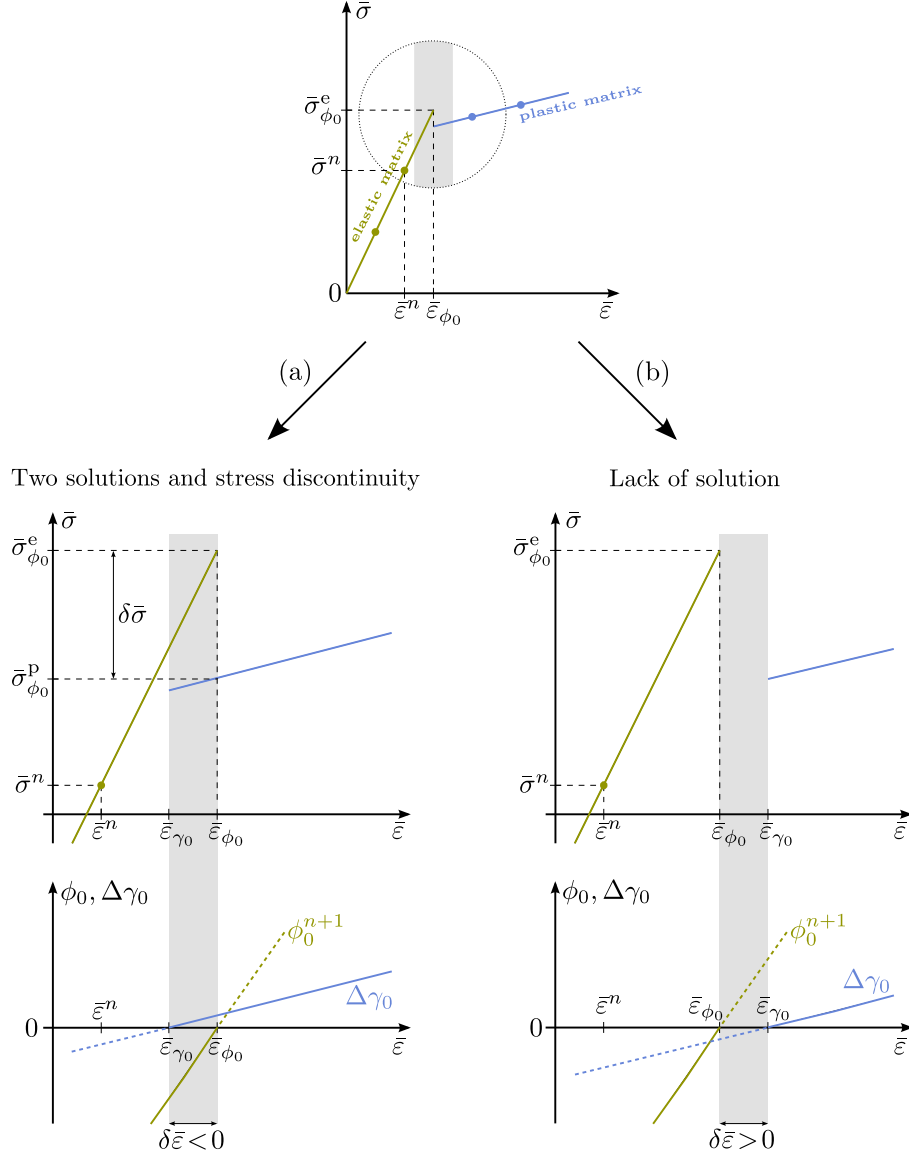
FIG. 2. Illustration of the response discontinuities at the elastic-to-plastic transition in the incremental Mori-Tanaka scheme. See text for explanations.
