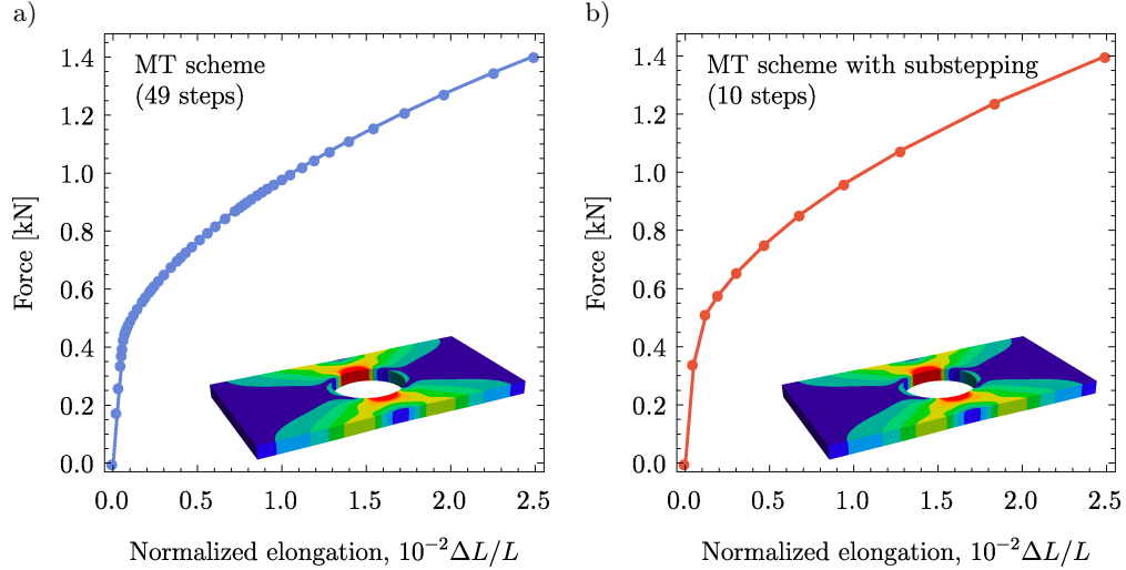
FIG. 1. Illustration of the impact of response discontinuities on the convergence behavior and robustness of the incremental MT scheme employed in finite element computations: a) basic MT scheme exhibiting severe convergence problems that are caused by the discontinuities; b) MT scheme enhanced by a substepping strategy that eliminates the discontinuities. The diagrams present the force–displacement curves with dots indicating the load steps for the problem of tension of a rectangular composite block with a hole, cf. [39].
