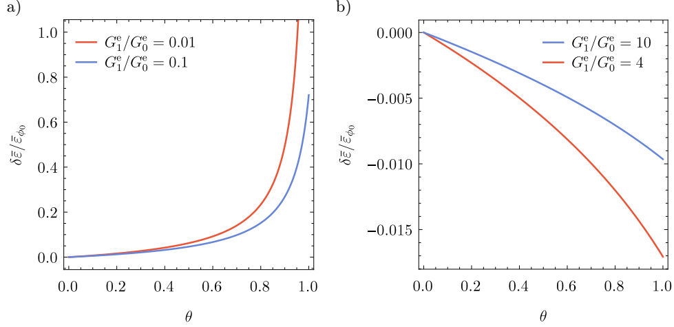
FIG. 7. Normalized strain gap \delta\bar{\varepsilon}/\bar{\varepsilon}_{\phi_0} as a function of parameter \theta for the fixed ratio of elastic shear moduli and for H_0/G_0^e = 0.008 .
