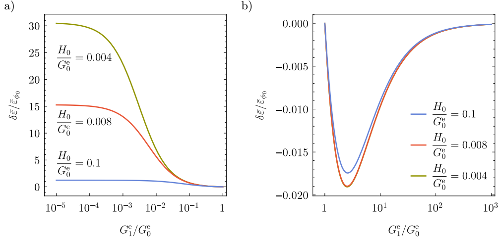
FIG. 3. Normalized strain gap \delta\bar{\varepsilon}/\bar{\varepsilon}_{\phi_0} as a function of the ratio of elastic shear moduli: a) G_1^e/G_0^e \leq 1 and b) G_1^e/G_0^e \geq 1 .
