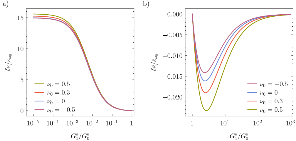
FIG. 4. Effect of Poisson's ratio \nu_0 on the normalized strain gap \delta\bar{\varepsilon}/\bar{\varepsilon}_{\phi_0} for a) G_1^e/G_0^e \leq 1 and b) G_1^e/G_0^e \geq 1 .
