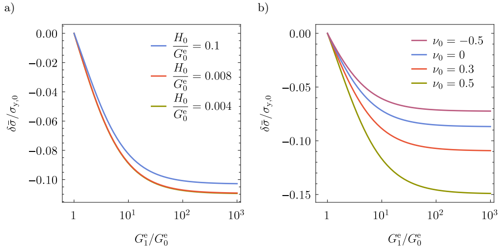
FIG. 5. Normalized stress jump \delta\bar{\sigma}/\sigma_{y,0} as a function of the elastic shear moduli ratio G_1^e/G_0^e \geq 1 . The effect of the normalized hardening coefficient H_0/G_0^e (a) and Poisson's ratio \nu_0 (b) is also shown.
