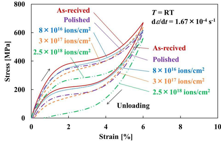
FIG. 1. Stress-strain curves.
