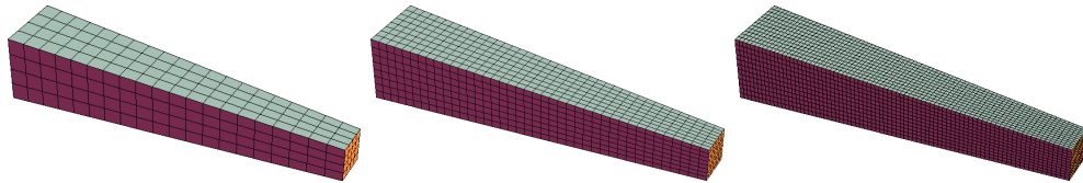
FIG. 2. Discretizations of VCSB: 20 \times 4 \times 4 (coarse mesh), 40 \times 8 \times 8 (medium mesh) and 80 \times 12 \times 12 (fine mesh).
