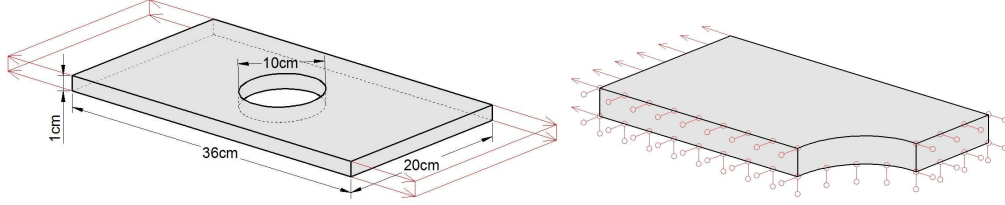
FIG. 3. Geometry and boundary conditions for PP.
