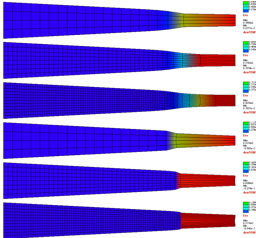
FIG. 8. Deformed meshes at the end of tension test with E_{xx} distribution for material averaging (upper three pictures) and spatial averaging (lower three pictures) – hyperelasticity-gradient-damage, VCSB.
