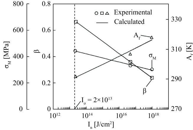
FIG. 9. Dependence of A_f , \sigma_M and \beta on I_n .
