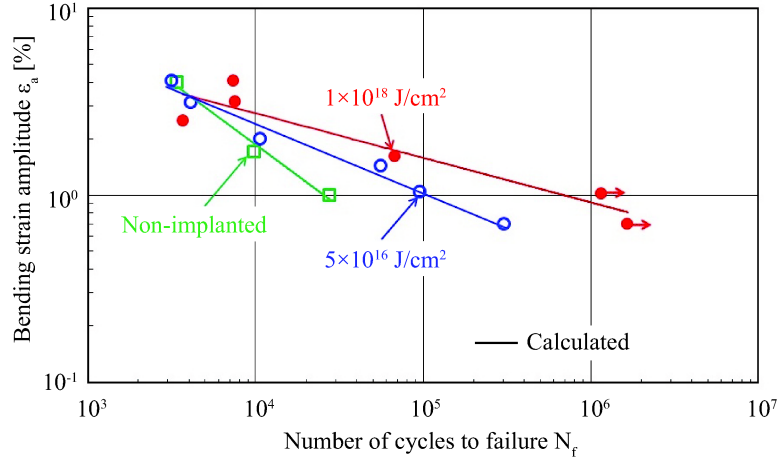
FIG. 4. Relationship between bending strain amplitude and the number of cycles to failure obtained by alternating-plane bending fatigue test.
