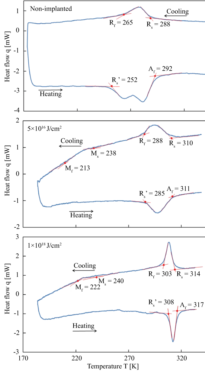
FIG. 2. DSC curves of ion-implanted and non-implanted SMA wires.
