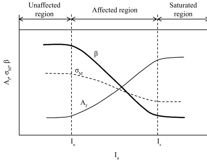
FIG. 8. Schematic dependence of A_f , \sigma_M and \beta on I_n .
