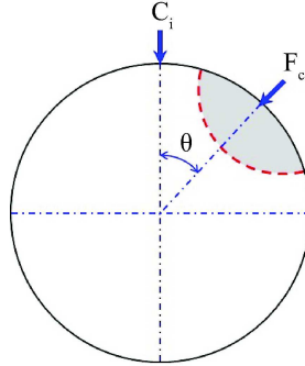
FIG. 6. Angle \theta at crack initiation point F_c from the maximum bending strain point C_i at the center of ion implantation.
