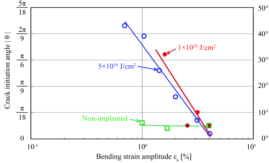
FIG. 7. Relationship between angle at crack initiation point |\theta| from maximum bending strain point at the center of ion implantation and bending strain amplitude \varepsilon_a .
