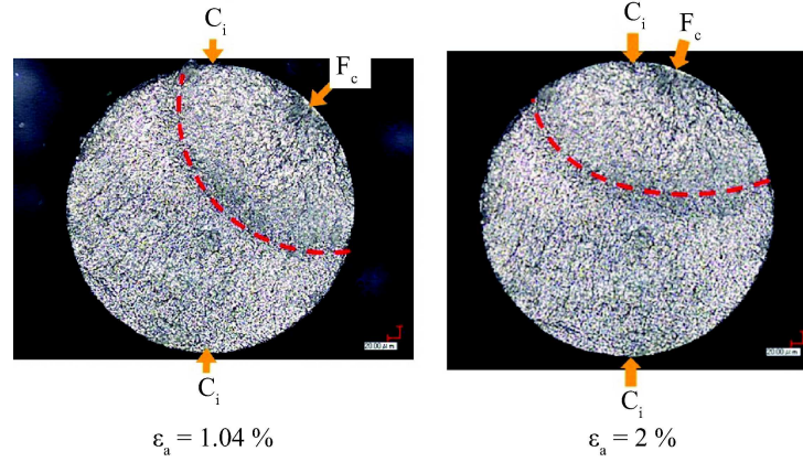
FIG. 5. Photographs of a fracture surface of the wire ion-implanted with 5 \times 10^{16} \text{ J/cm}^2 obtained by the fatigue test for \varepsilon_a = 1.04\% and 2\% . C_i is maximum bending strain point at the center of ion implantation, F_c is crack initiation point.
