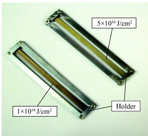
FIG. 1. View of ion implanted TiNi wire-samples in special holder.
