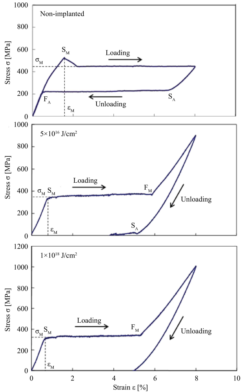
FIG. 3. Stress-strain curves of ion-implanted and non-implanted SMA wires.
