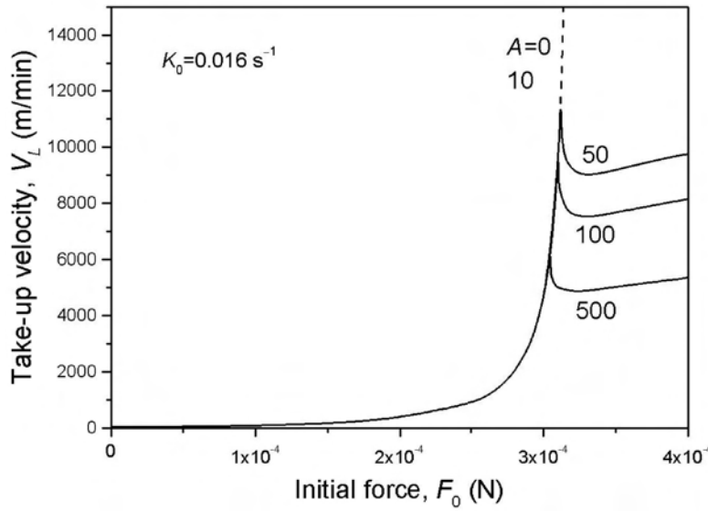
FIG. 7. Velocity-tension relations for crystallizing melts. Standard hyperbolic viscosity-crystallinity function combined with stress-induced crystallization. Thermal crystallization rate, K_0 = 0.016 \text{ s}^{-1} , stress-induced crystallization rate coefficients, A , indicated.
