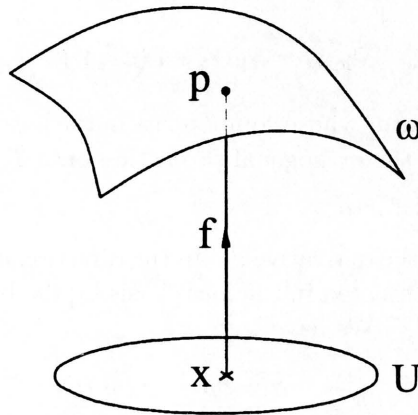
FIG. 2. Parametrization of the surface \omega .
